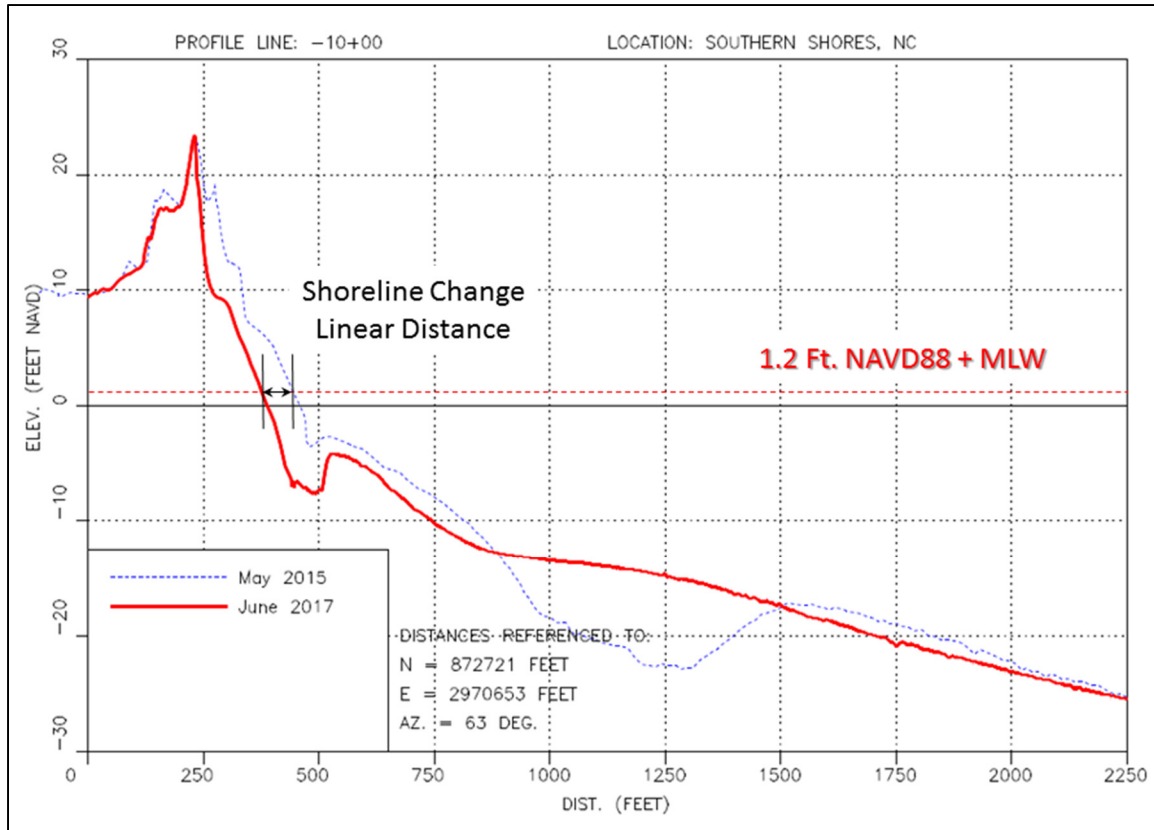
Figure 3. Beach profile cross section illustrating shoreline change.
