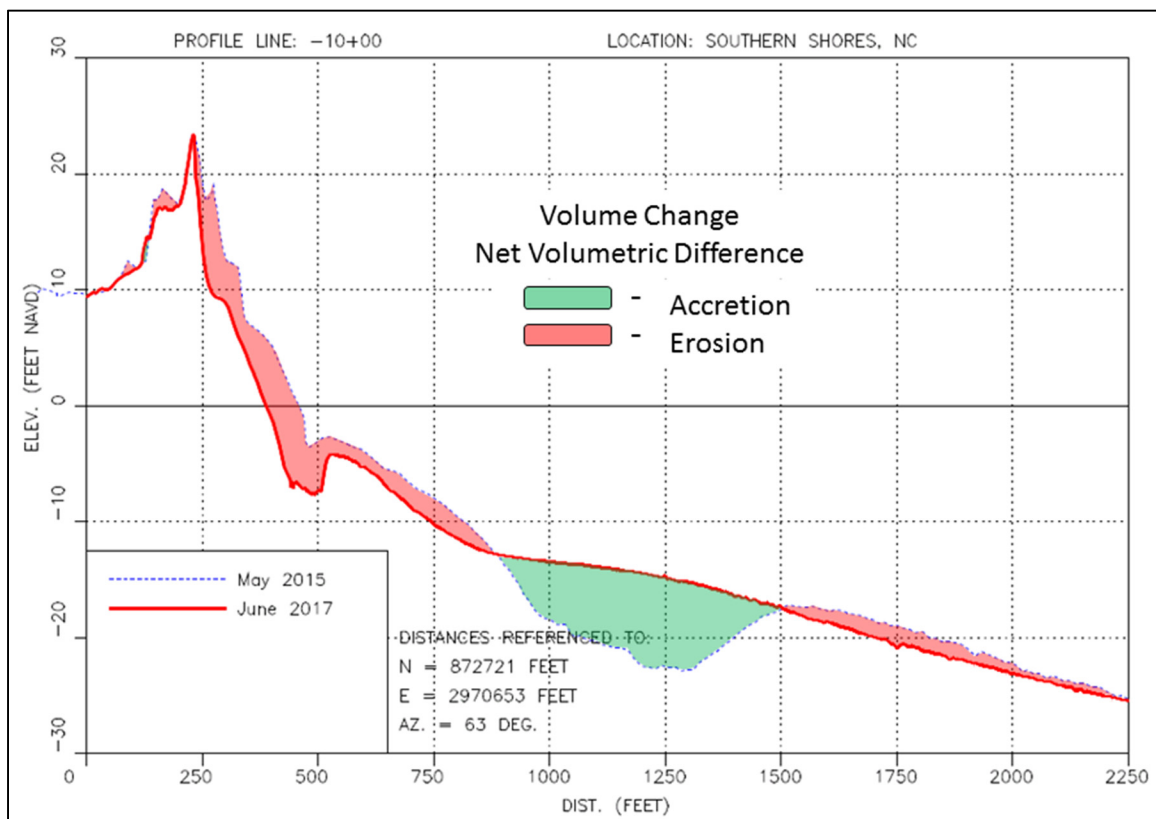
Figure 6. Beach profile cross section illustrating volume change.
