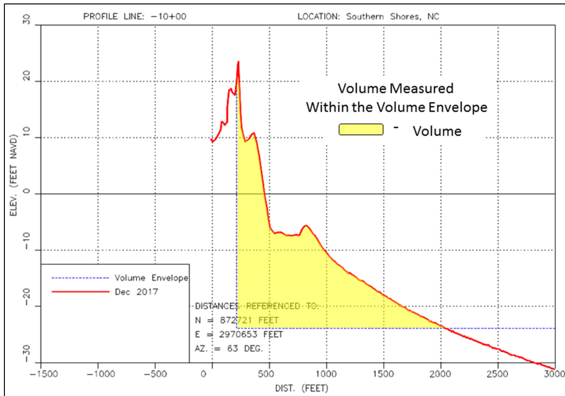
Figure 9. Beach profile cross section illustrating the volume envelope.
