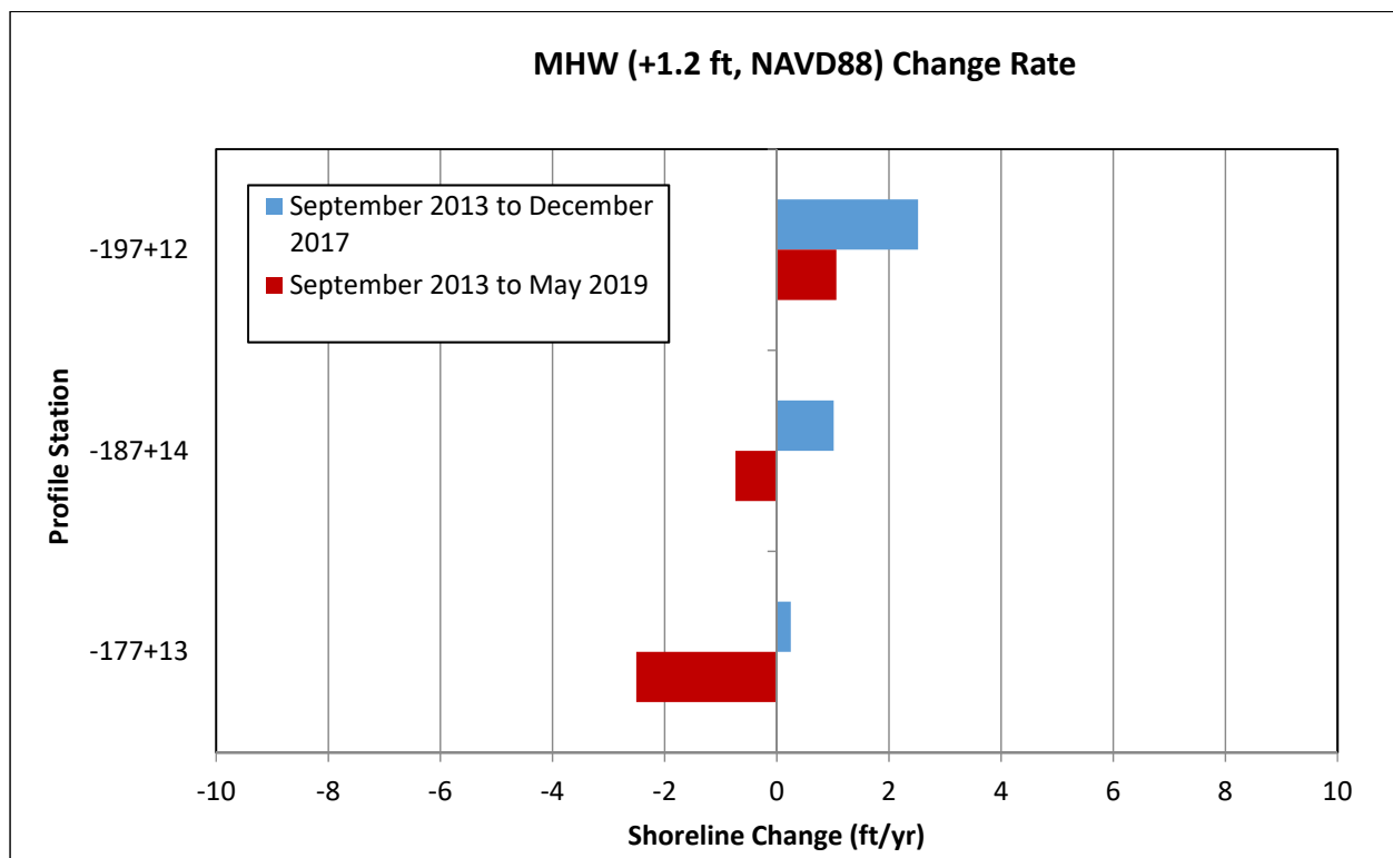
Figure 5. Average shoreline change rates measured from October 2006 to December 2017, and from October 2006 to May 2019.
