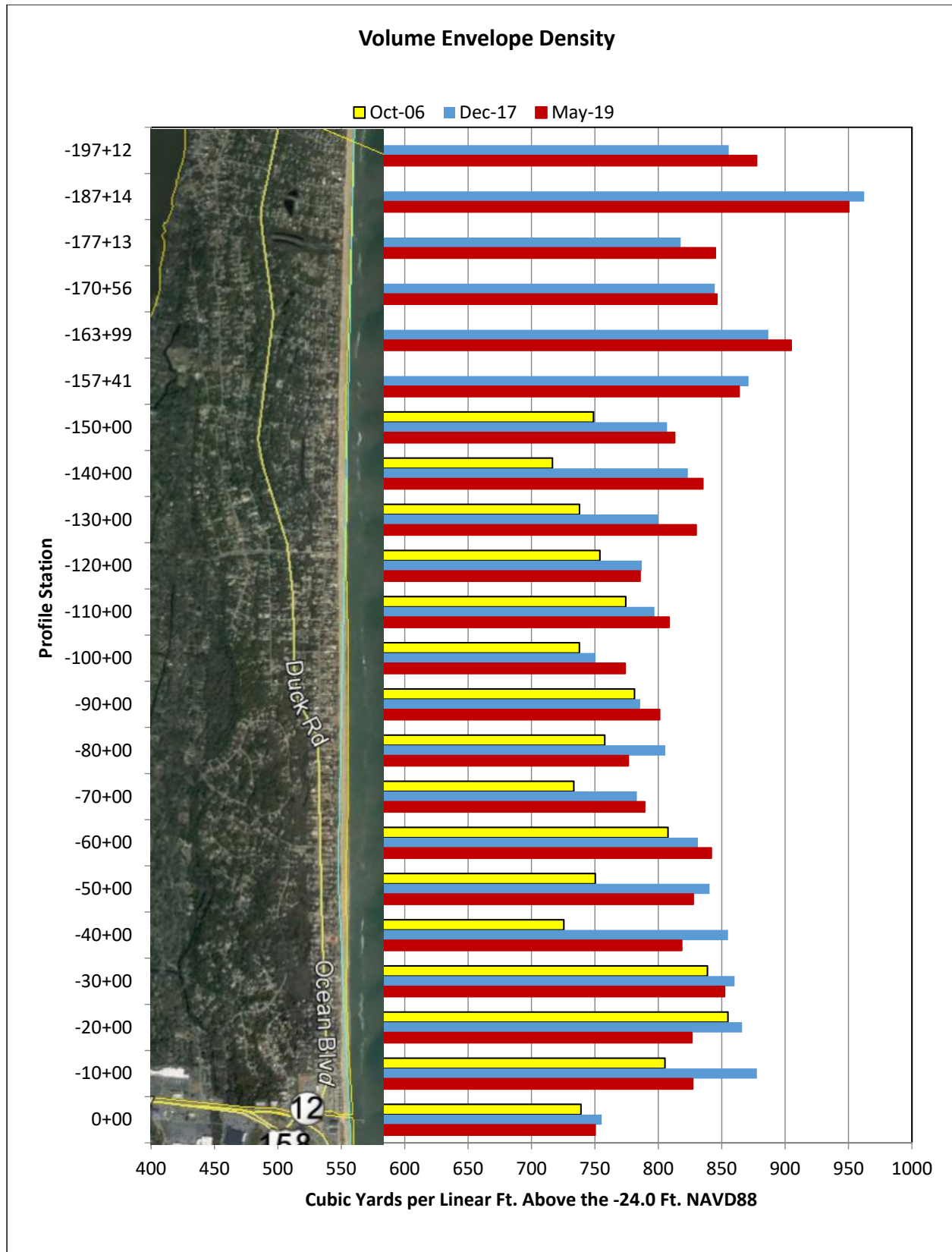
Figure 10. Volume envelope calculations across all Southern Shores profiles.
