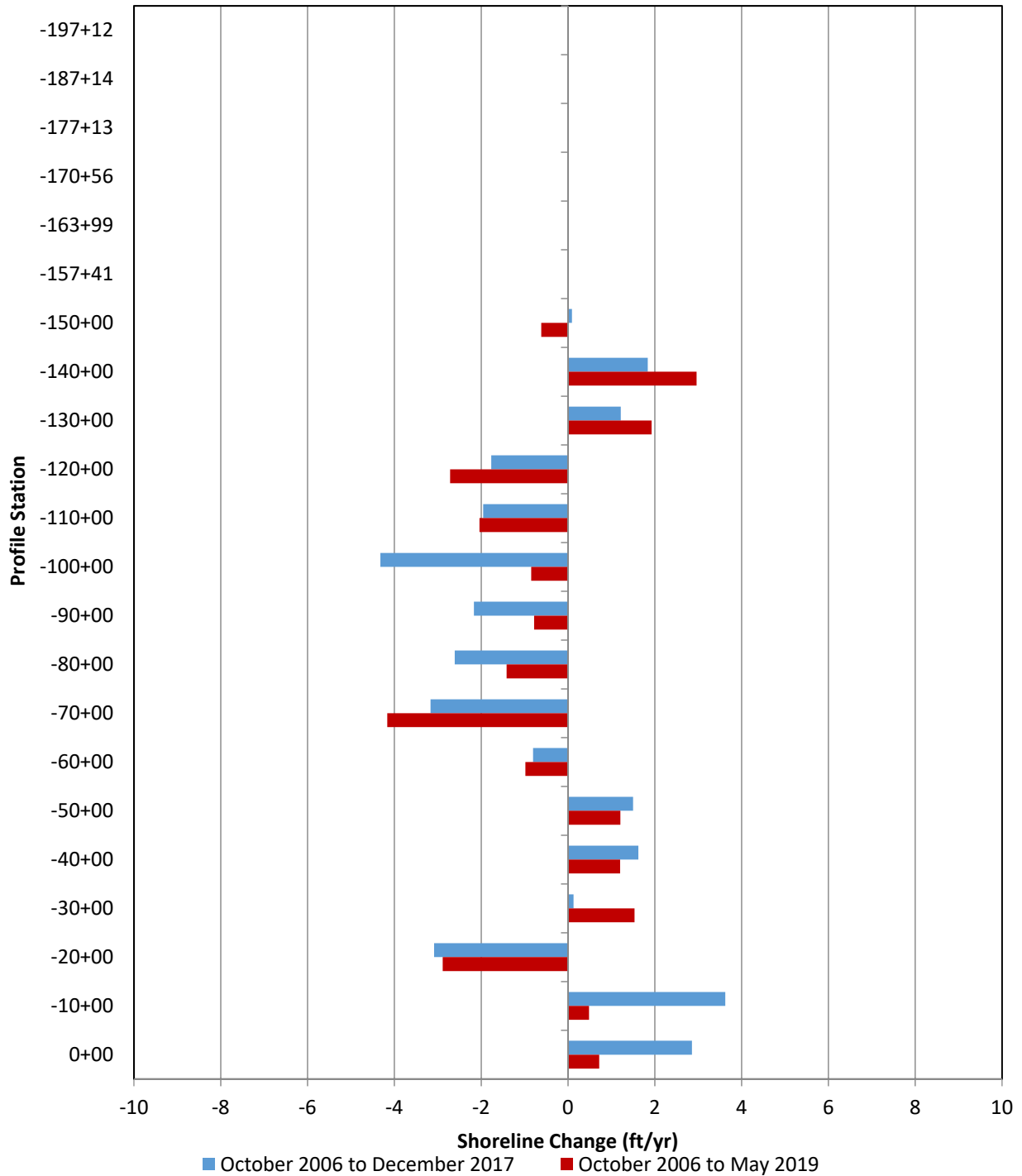
Figure 4. Shoreline change rates measured between October 2006 and December 2017, and October 2006 and May 2019.
