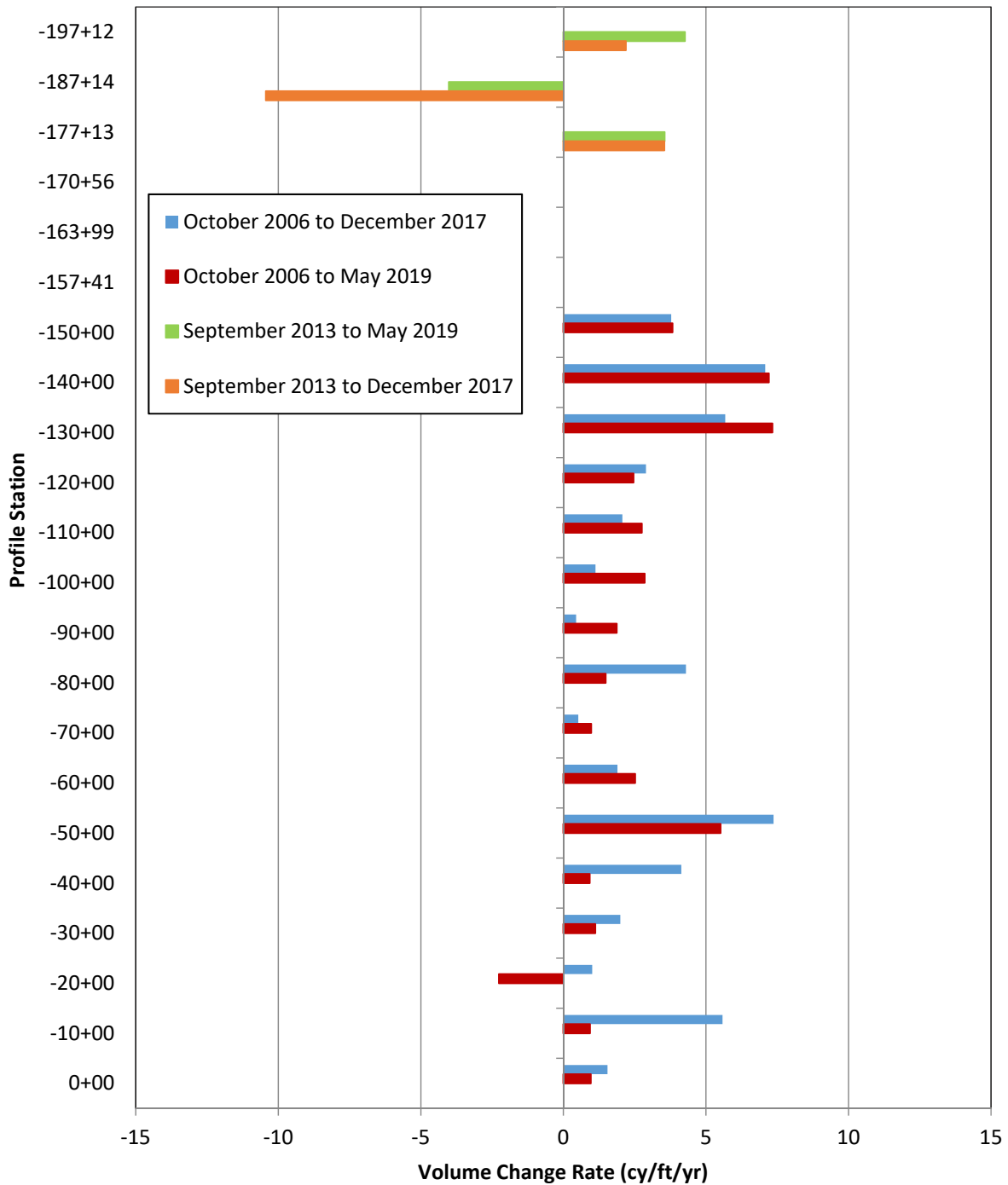
Figure 8. Long-Term Annual Volumetric Change Rate above -24 FT NAVD88 (CY/FT/YR)
